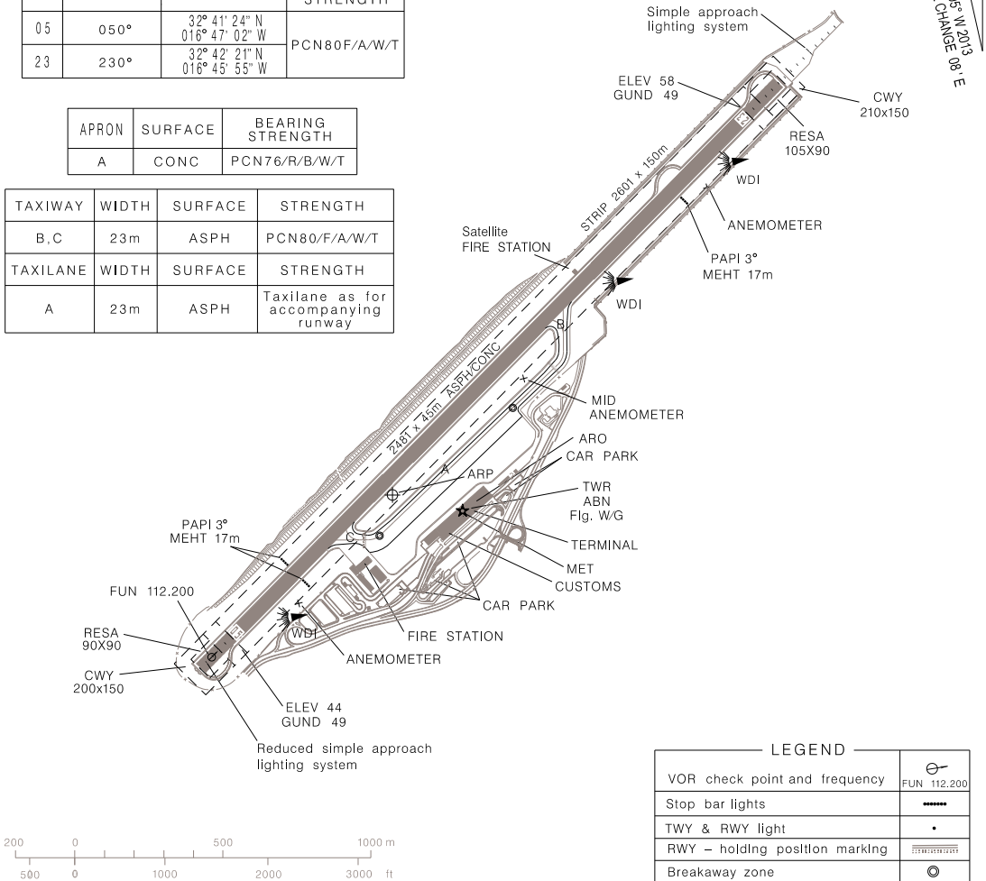
MARKING AIDS RWY 05/23 AND EXIT TWY
